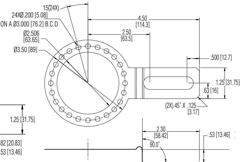
114574-0001 Slotted Tether Kit
