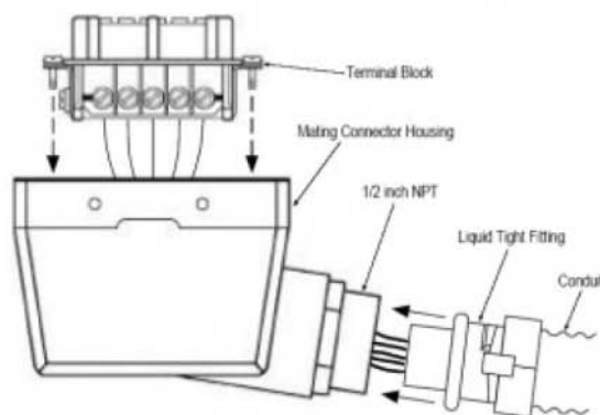
Figure 5: Sealed Industrial Latching Connector
