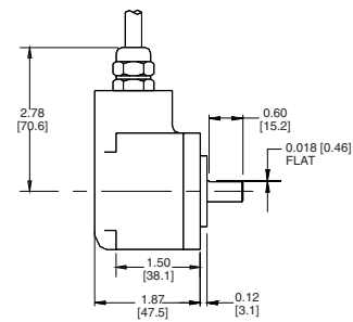
Cable Exit
